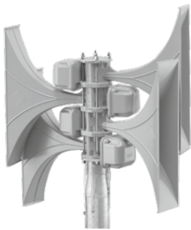
SIREN HEAD Siren head consisting of self-supporting siren horns in modular construction.
